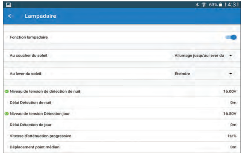
Screen on a tablet Settings of street light features
